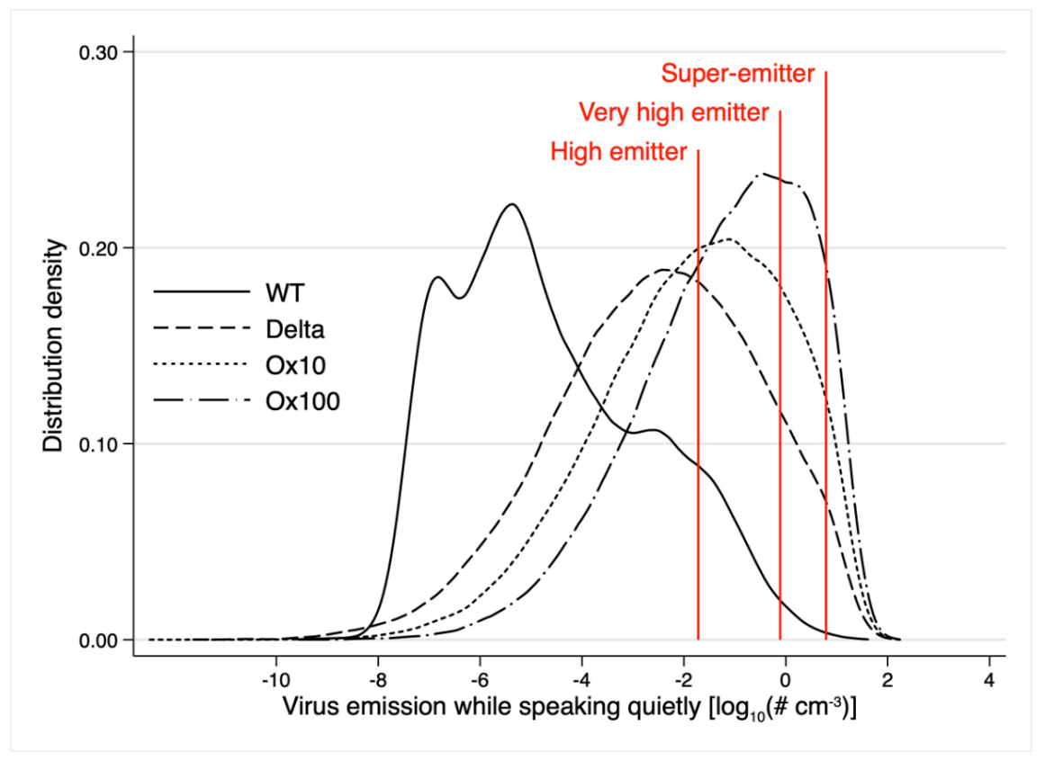
Figure 1: Distribution of viral emissions in populations infected with the WT, the Delta and the Omicron variants when speaking at low vocal intensity. Red lines indicate the high emitter (90 th percentile of WT), very high emitter (99 th ) and super-emitter (99.9 th ) thresholds. Ox10 and Ox100 indicate simulations for Omicron assuming 10 times and 100 times higher mean viral loads compared to Delta.
